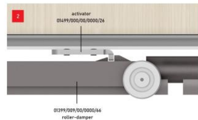
Door in closing phase. Damper loaded and to be activated 門正在關上，阻尼裝置裝入及準備啟動
