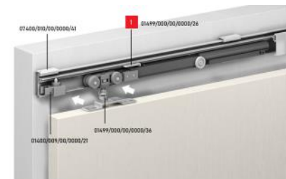
Side-wall fixing application example 壁裝安裝圖
