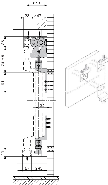
Each door panel operates on two top tracks and one bottom channel. 每扇門板操作於2條頂路軌及1條導向底路軌上
