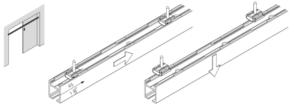
Dismounting the running track is simple and easy 移除路軌的方法簡單、容易
