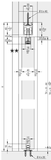
Efficient movement support with Push-to-Open with self-closing mechanism for the Hawa Porta 100 HMT Hawa Porta 100HMT 的自閉裝置能與按彈裝置同時使用，提供高效能移動
