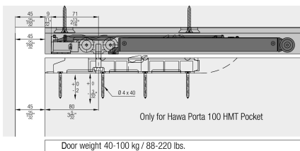
Push-to-open with self-closing mechanism: 按彈開啟連自閉裝置
