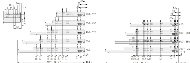
Fixing positions for full extension drawer 全拉出抽屜趟路鑽孔尺寸、跟櫃體前端尺寸
