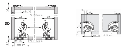
Locking device & adj. adapter fixing position 抽屜扣碼及調節碼安裝位置
