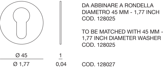
E. BOCCHETTA TONDA SLIM FORO CILINDRO DIAMETRO 45 MM - 1,77 INCH ROUND SLIM CYLINDER HOLE ESCUTCHEON DIAMETER 45 MM - 1,77 INCH
