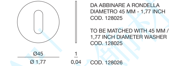
D. BOCCHETTA TONDA SLIM FORO CHIAVE DIAMETRO 45 MM - 1,77 INCH ROUND SLIM KEY HOLE ESCUTCHEON DIAMETER 45 MM - 1,77 INCH
